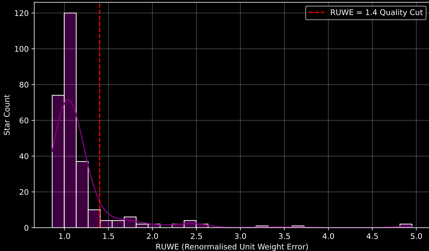
GALAH DR4 Field [9161] RUWE Distribution (n= 271)
