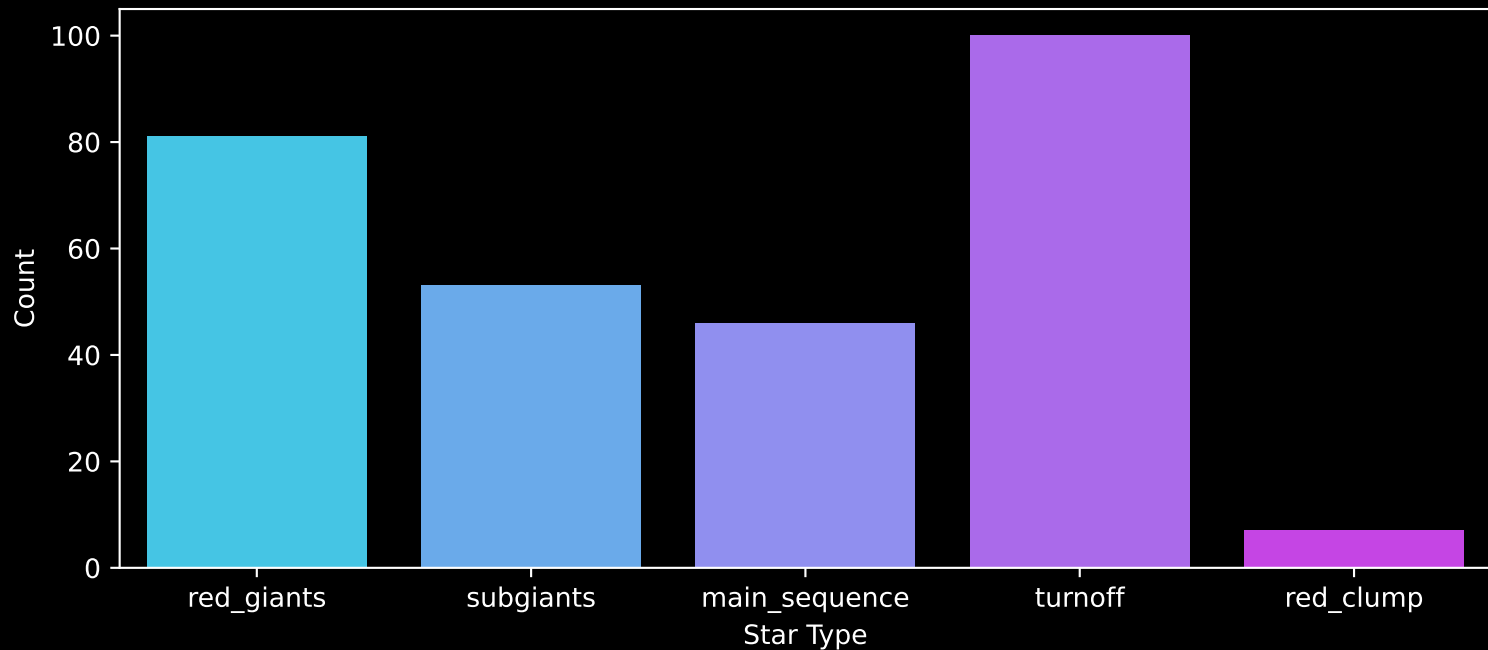
GALAH DR4 Field: [9161] Count plot of Star Type
