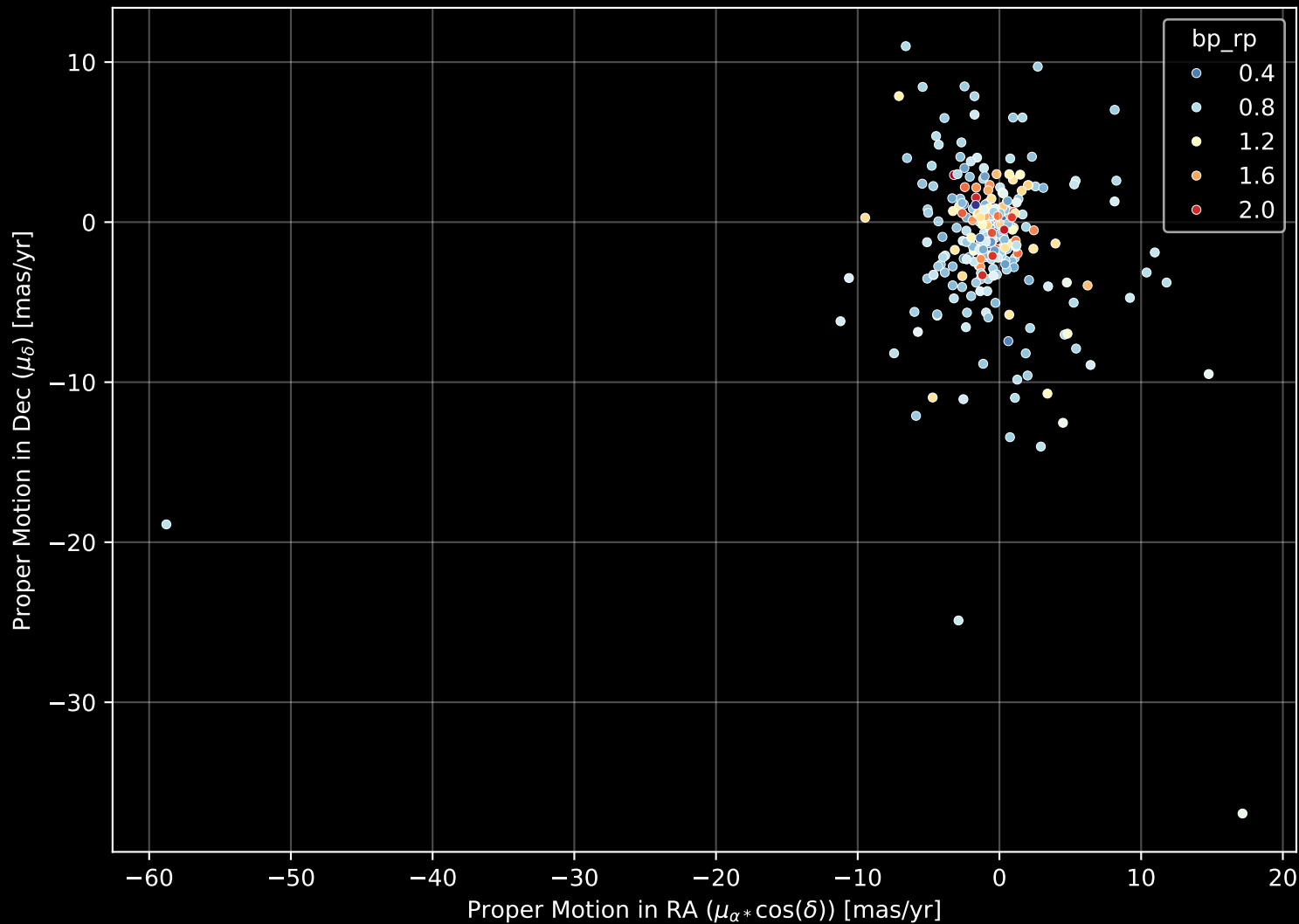
GALAH DR4 Field: [9161] Proper Motion Diagram (n= 287)
