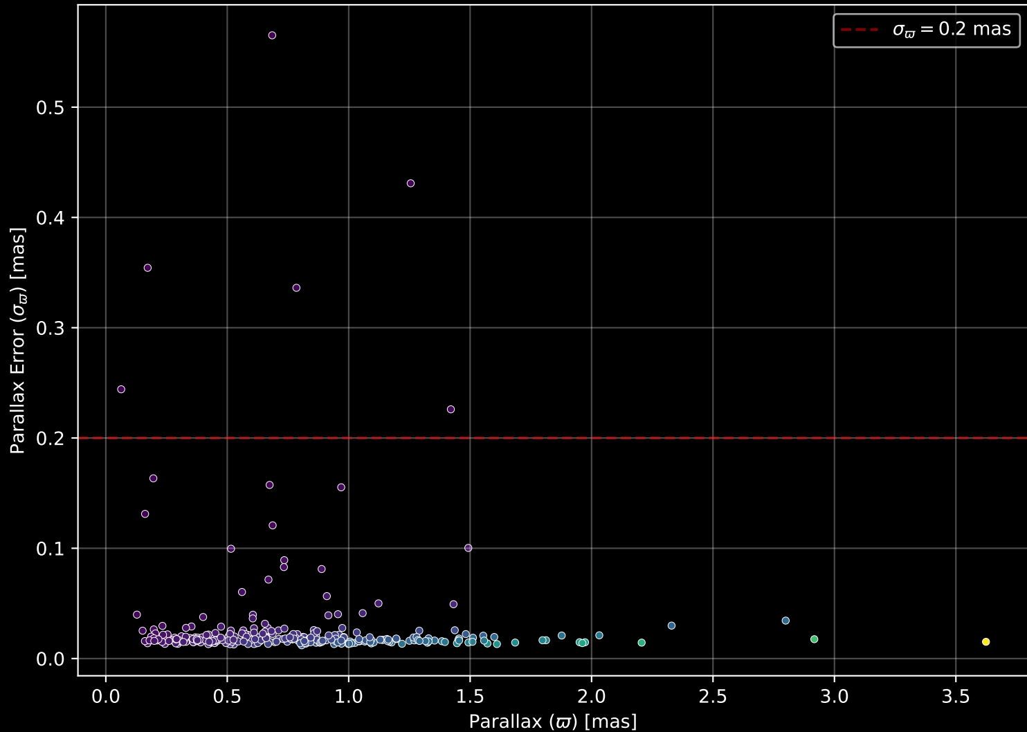
GALAH DR4 Field: [9161] Parallax Quality (n= 287)
