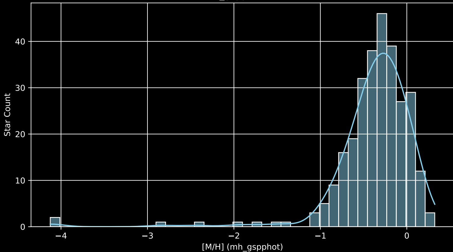
GALAH DR4 Field: [9161] [M/H] (mh_gspphot) (n= 286)
